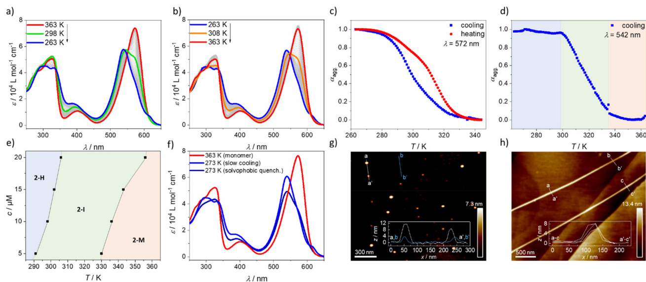
Fig. 2 UV-vis cooling (a) and heating (b) experiments of 2 (MCH, 10 \mu\text{M} , 1 K \text{min}^{-1} ) with the corresponding cooling and heating curves, plotted at \lambda = 572 nm (c). (d) Cooling curve of 2 plotted at \lambda = 542 nm to demonstrate the two-step process (MCH, 10 \mu\text{M} , 1 K \text{min}^{-1} ). (e) Phase diagram extracted from cooling experiments of 2 at different concentrations. (f) UV-Vis experiments depicting the solvophobic quenching of 2 (10 \mu\text{M} , MCH/ \text{CHCl}_3 ). (g) AFM image of 2-I after spin-coating a 20 \mu\text{M} solution of 2 (306 K, MCH) on HOPG and (h) AFM image of 2-H after spin-coating a 20 \mu\text{M} solution of 2 (273 K, MCH) on HOPG.
