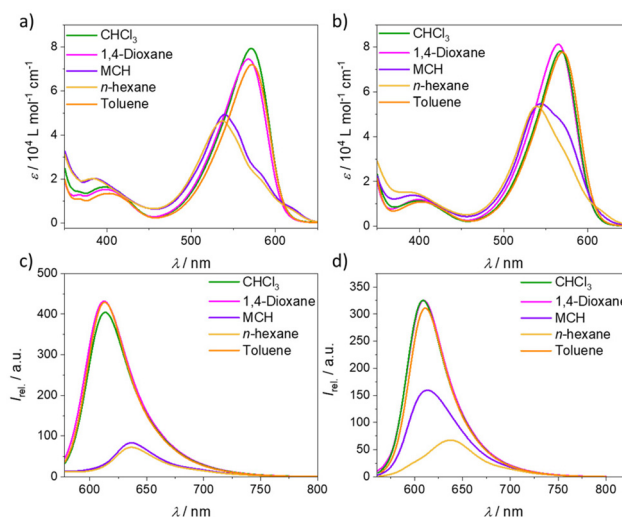
Fig. 1 Solvent-dependent UV-vis and emission studies ( \lambda_{exc.} = \lambda_{max. abs.} ) of 1 (a and c) and 2 (b and d) at c = 10 \mu\text{M} at room temperature.
