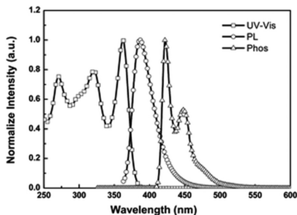
Fig. 5 UV-vis absorption, fluorescence spectra of CZ-ArB-8 in DCM solution and the phosphorescence spectra at 77 K in EtOH. Reproduced with permission from ref. 104. Copyright 2012 Royal Society of Chemistry.
