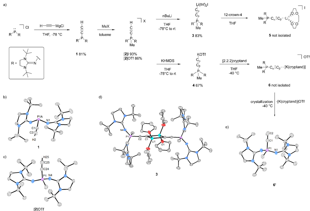
Fig. 3 (a) Synthesis of the alkali metal phosphonioacetylide complexes 3–6. Solid-state structures of (b) 1, (c) [2]OTf , (d) 3 and (e) 6'. Hydrogen atoms except the hydrogen attached at C_\beta and counter ions (triflate for [2]OTf , iodide for 3) are omitted for clarity. Ellipsoids are displayed at 50% probability. Selected structural data is shown in Table 1.
