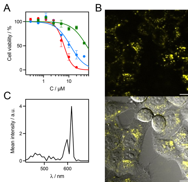
Fig. 8 (A) MTT proliferation assays performed on HeLa cells with dTAT [Eu-L-Ar-NHAc] (green), 19 dTAT[Eu-L-Ar-Ar-NHAc] (blue) and dTAT [SucNH-Ar-Ar-L-Eu] (red). (B) 2PM imaging ( \lambda_{\text{ex}} = 720 \text{ nm} ) of HeLa cells incubated 1 h with dTAT[SucNH-Ar-Ar-L-Eu] ( 2 \mu\text{M} ) in RPMI medium, showing (top) the luminescence image recorded with 420–680 nm bp APD detection and (bottom) the superimposition of DIC and luminescence images. (C) Typical emission spectrum emanating from puncta. Scale bars correspond to 10 \mu\text{m} .
