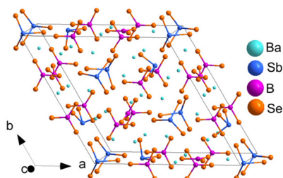
Fig. 5 The structure of \text{Ba}_3(\text{BSe}_3)(\text{SbSe}_3) .
