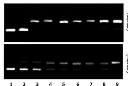
Fig. 4 Agarose gel electrophoresis images of pBR322 plasmid DNA ([DNA]bp = 15 μM) incubated with decreasing concentrations (20–0.1 μM) of 1 (top) and 2 (bottom) for 1 h minutes at 37 °C. Lane 1: DNA control; lanes 3–9: DNA and complexes at concentrations 0.1, 0.5, 1, 2.5, 5, 10, 15, 20 μM.
