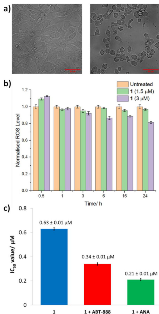
Fig. 7 (a) Representative bright-field images ( \times 20 ) of untreated HMLER-shEcad cells (left) and HMLER-shEcad cells treated with 1 ( 4 \times \text{IC}_{50} value for 24 h, right). (b) Normalised ROS activity in untreated HMLER-shEcad cells and HMLER-shEcad cells treated with 1 ( 4 \times \text{IC}_{50} value for 0.5, 1, 3, 6, 16, and 24 h). Error bars represent standard deviations. (c) Graphical representation of the \text{IC}_{50} values of 1 towards HMLER-shEcad cells in the absence and presence of ABT-888 (10 \mu\text{M} ) or ANA (10 \mu\text{M} ). Error bars represent standard deviations.
