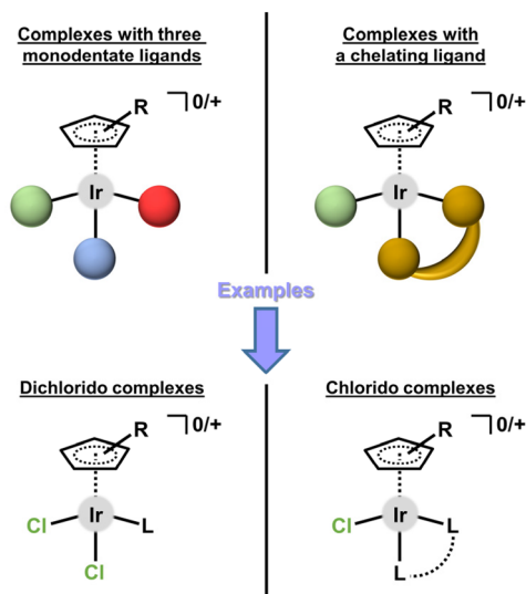
Fig. 3 Two basic structural types of half-sandwich iridium(III) cyclopentadienyl complexes ( \text{Ir-Cp}^{\text{x}} ).
