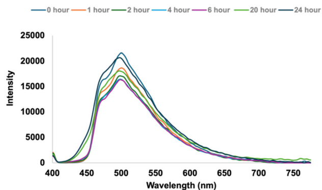
Fig. 4 Emission spectral overlay of aliquots drawn during the alkyne-alkene cycloaddition, catalyzed by IrCat1. For each sample, 100 \mu\text{L} of the reaction mixture was diluted to 500 \mu\text{L} in DCM, followed by recording a spectrum. While some small changes to the emission intensity are noted, the intensity prior to the reaction (0 hour trace) and at the conclusion of the reaction (24 hour trace) are nearly identical, suggesting the photocatalyst maintains high fidelity throughout the course of the reaction.
