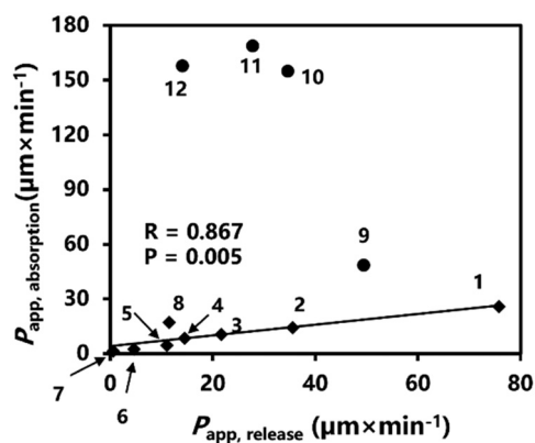
Fig. 2 Correlation between P_{app, absorption} and P_{app} and the release of compounds. The line indicates the linear regression for hydrophilic compounds. 1, 5-FU; 2, PHBA; 3, PSP; 4, BPB; 5, BSP; 6, FD-4; 7, FD-10; 8, DOX; 9, antipyrine; 10, methylparaben; 11, propylparaben; and 12, butylparaben. Diamonds and circles indicate hydrophilic and lipophilic compounds, respectively.
