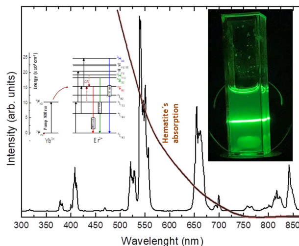
Fig. 4 Up-conversion emission spectrum of solvothermal \text{NaYF}_4\text{:}5\%\text{Yb}^{3+}\text{-}2\%\text{Er}^{3+} micro-sized particles under excitation with a 980 nm laser diode with a power of up to 300 mW. The inset shows the energy level diagrams of \text{Yb}^{3+} and \text{Er}^{3+} ions with the main emission transitions labelled with the corresponding wavelengths. Also shown is a photograph of up-conversion solvothermal microparticles under infrared excitation. Hematite's absorbance curve is depicted by a red solid line as a reference to demonstrate the perfect overlap with the green up-conversion emission spectrum from the rare-earth-doped \text{NaYF}_4 particles.
