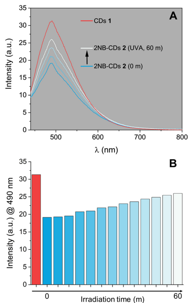
Fig. 3 (A) Emission spectra ( 10 \mu\text{g mL}^{-1} , 20^\circ\text{C} , \text{H}_2\text{O} , \lambda_{\text{ex}} = 420 nm, blue traces) of 2NB-CDs 2 before and after ultraviolet irradiation (365 nm, 0, 20, 40 and 60 min). The red trace is the emission of unfunctionalized CDs 1 recorded under identical concentration and excitation conditions. (B) Evolution of the emission intensity at 490 nm of 2NB-CDs 2 ( 10 \mu\text{g mL}^{-1} , 20^\circ\text{C} , \text{H}_2\text{O} , \lambda_{\text{ex}} = 420 nm, blue bars) recorded before and after ultraviolet illumination (0–60 m, 5 min intervals). The red bar is the emission at 490 nm of unfunctionalized CDs 1 recorded under identical concentration and excitation conditions.
