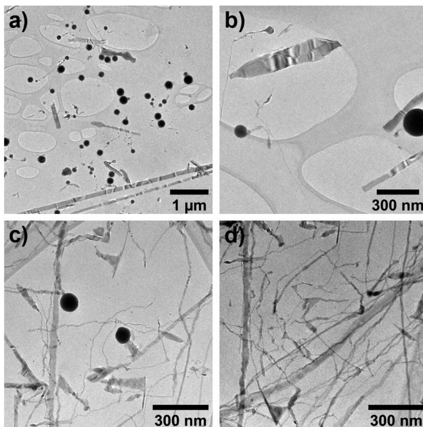
Fig. 3 TEM images of variations on the InP nanowires with 10 (a and b) or 50 (c and d) mole % extra P(\text{NEt}_3)_3 .
