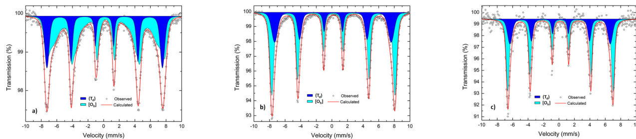
Fig. 4 The room-temperature ^{57}\text{Fe} Mössbauer spectra of (a) HEOFe, (b) LiHEOFeF, and (c) LiHEOFeCl. The dark blue and light blue spectra correspond to tetrahedrally ( T_d ) and octahedrally ( O_h ) coordinated iron cations, respectively.
