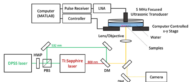
Fig. 4 Schematic illustration of the photoacoustic microscope (PAM) working at 532 and 800 nm. HWP: half-wave plate, PBS: polarizing beam splitter, DM: dichro mirror, LNA: low-noise amplifier.
