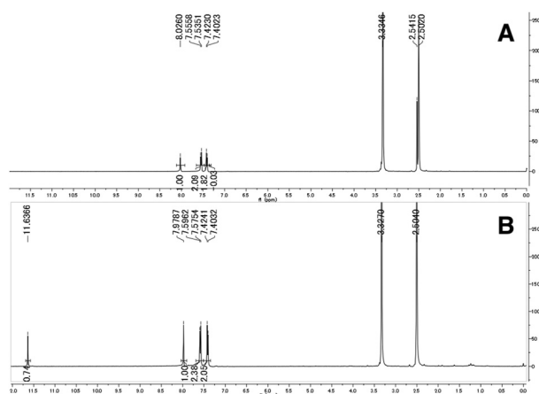
Fig. 3 Selected ^1\text{H} -NMR spectra of 2f (A) and \text{Zn}(\text{2f})_2 (B) in dimethyl sulfoxide- \text{d}_6 .
