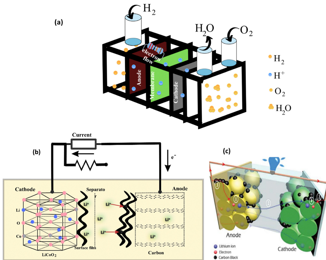
Fig. 17 (a) Diagram of a basic fuel cell. (b) Schematic of a typical lithium-ion battery featuring a graphite anode and a LiCoO 2 cathode. (c) Illustration of lithium-ion and electron transport routes during the battery discharge process. Reproduced from ref. 100 with permission from Royal Society of Chemistry, copyright 2019.
