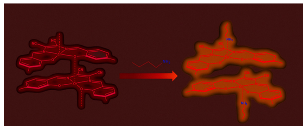
Fig. 21 Vapochromic behaviour shown by ML 12 for n -butylamine; reproduced from ref. 131 with permission from Elsevier. Copyright 2024.
