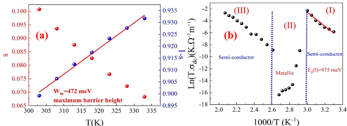
Fig. 13 (a) Temperature variation of the exponents “ s ” and “ 1 - s ” within the temperature range of 303–333 K (b) Plot of \ln(\sigma_{dc} T) as a function of (1000/T) within the temperature range of 303–490 K for the eco-friendly synthesized CFO nanoparticles.
