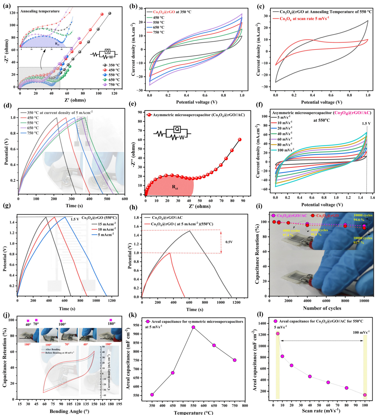
Fig. 6 (a) Impedance analysis for CR-1 to CR-5 at different annealing temperatures. (b) CV performance of CR-1 to CR-5 at 5 mV s -1 . (c) Comparison of pristine \text{Co}_3\text{O}_4 and \text{Co}_3\text{O}_4/\text{rGO} at 550 °C. (d) GCD analysis, (e) EIS of the asymmetric device, (f) CV of the asymmetric device at 550 °C, (g) GCD of the asymmetric device, (h) comparative analysis for GCD. (i) Show the capacitance retention over various cycles, (j) flexibility curve of the device, (k) shows the areal capacitance for the symmetric microsupercapacitor at 5 mV s -1 , and (l) shows the areal capacitance for the asymmetric microsupercapacitor for various scan rate.
