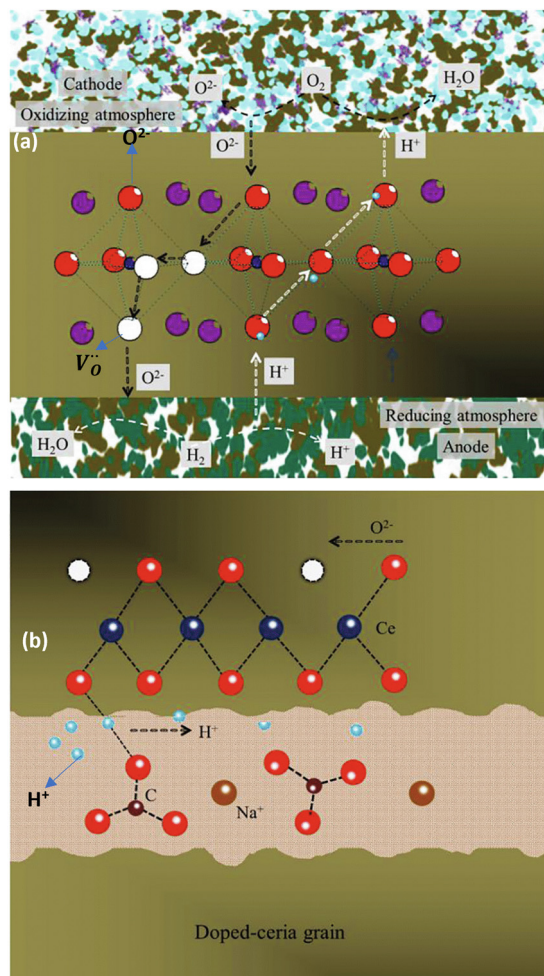
Fig. 11 (a) Schematic model of mixed conduction for single perovskite-based electrolyte. (b) Schematic model of SDC/Na _2 CO _3 nanocomposite. 213,216 Reproduced from ref. 213 with permission from [Elsevier], copyright [2021].
