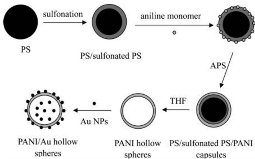
Figure 11 Scheme of the preparation of PANI and PANI/Au hollow spheres. 210 Reproduced with permission from ACS.
