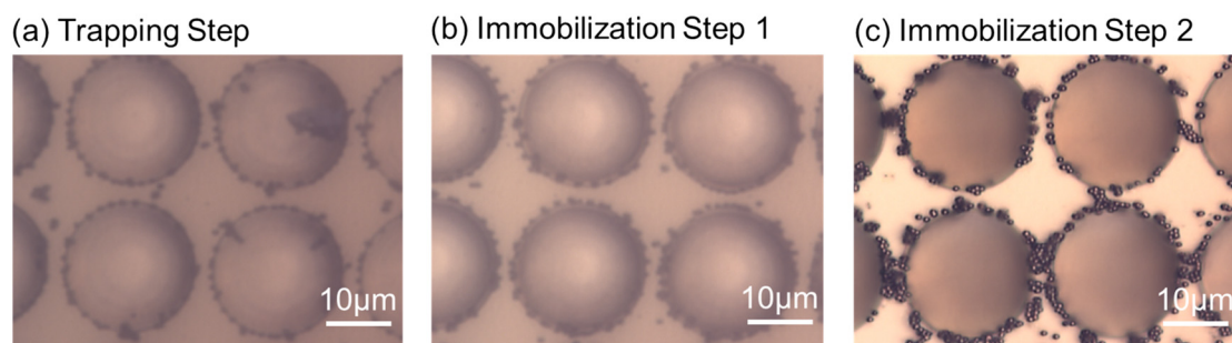
Fig. 4 Optical images of the particle immobilization step. (a) Represents the trapping step, (b) represents the immobilization step using the capacitance effect, while (c) represents the immobilization step using a positive current, measured in a dried state. All scale bars are 10 \mu\text{m} . The following are conditions of each step (a) 20 V_{pp} , 1 MHz. (b) 20 V_{pp} , 1 kHz. (c) 3 V_{pp} , 1 MHz with a +3 V DC offset.
