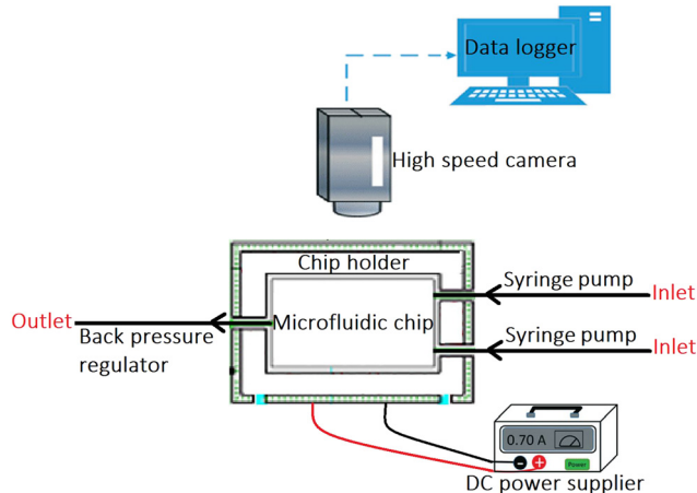
Fig. 1 Diagram of the HP-HLT microfluidic platform.
