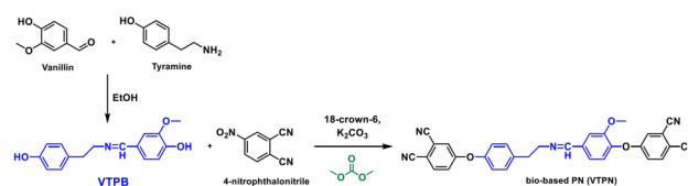
Scheme 33 Synthesis of a bio-based phthalonitrile (PN) resin (VTPN) via the nucleophilic substitution reaction between 4-nitrophthalonitrile and Schiff base bisphenol (VTBP). VTPB was obtained by reacting vanillin and tyramine in ethanol. 202
