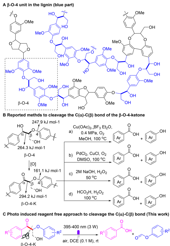
Scheme 1 Representative \beta -O-4 unit in the lignin skeleton and different approaches to the selective C( \alpha )-C( \beta ) bond cleavage of the \beta -O-4 model compound.
