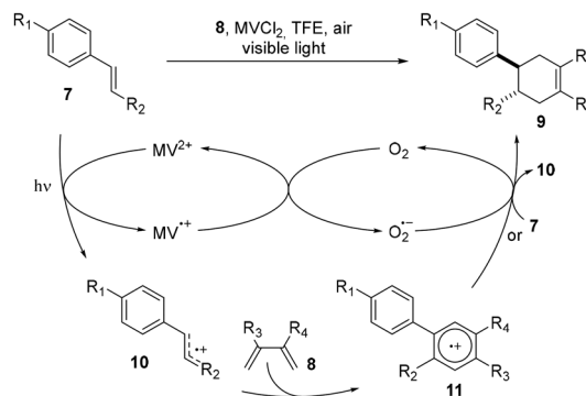
Scheme 4 Proposed mechanism.
