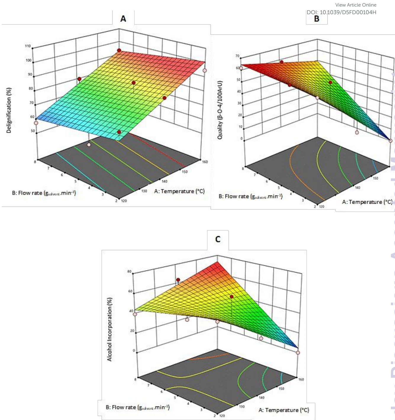
Figure 8. RSM 3D Models showing the effects of extraction temperature and flow-rate on investigated responses; (A)-Delignification Efficiency, (B)-Lignin Quality & (C)-Alcohol Incorporation
