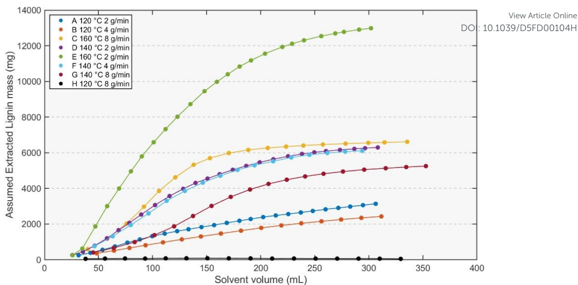
Figure 4. Plot of accumulated lignin mass vs. solvent use from the UV-Vis spectrophotometric monitoring of the flow-through extraction kinetics calibrated using an extinction coefficient obtained from a reference isolated birch lignin.
