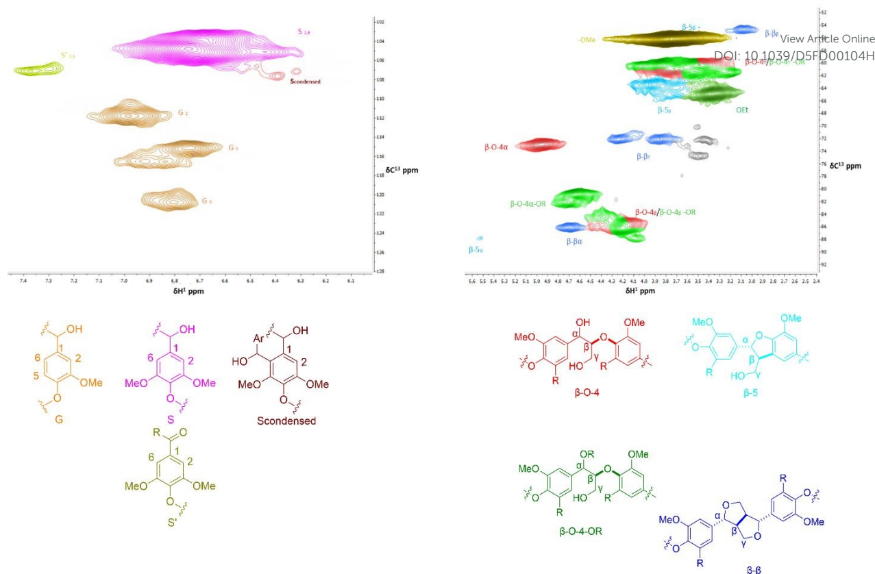
Figure 6. 2D-HSQC NMR of Organosolv extracted birch wood lignin showing the lignin aromatic subunit region (left) and linking motifs region (right) for Run B (120 °C, 4 g_{\text{solvent}} \cdot \text{min}^{-1} ) done in Acetone d_6 .
