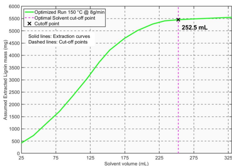
Figure 9. Plot of Accumulated Lignin Mass vs Solvent use with Solvent cut-off point for the optimized Run 150 at 8 \text{g}_{\text{solvent}}\cdot\text{min}^{-1}
