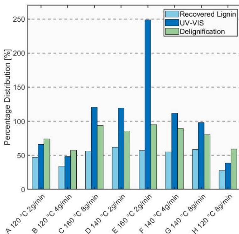
Figure 5. Comparison of lignin extraction obtained from different processing conditions including; lignin recovery from the purification process (Recovered Lignin), lignin yield from calibrated UV-Vis and lignin yield calculated based on the lignin content in the extraction residue (Delignification).
