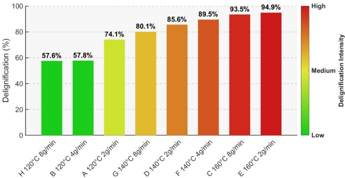
Figure 3. Delignification based on the compositional analysis on the crude biomass and the pulp obtained after lignin extraction (See SI Table S2 for details on quantified lignins based on the mass balance)
