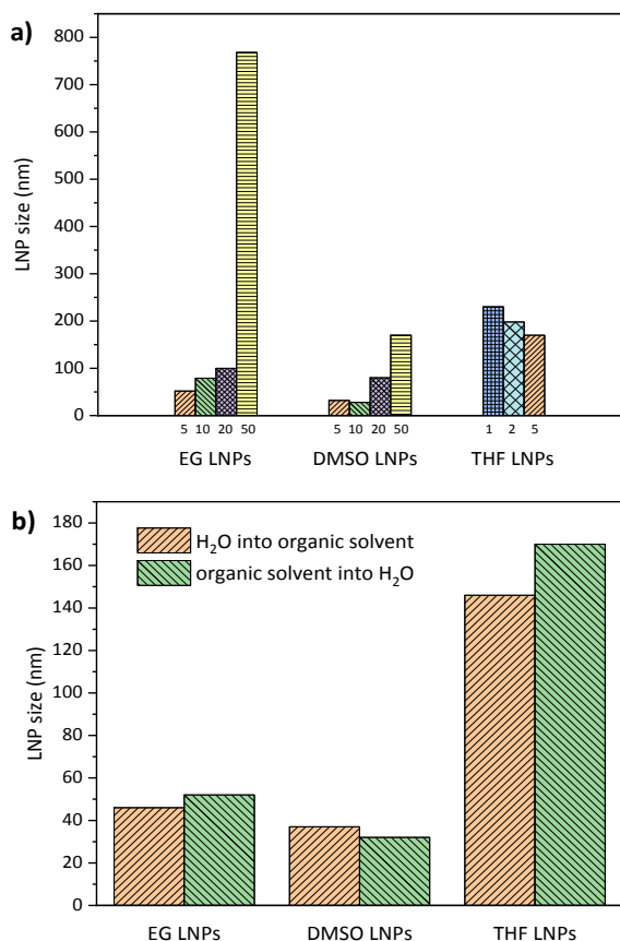
Figure 1: a) variation of the LNPs size as a function of the initial concentration of lignin (1, 2, 5, 10, 20, 50 mg mL -1 ). Data from the non-controlled (i.e. extremely fast) addition of the lignin solution into water. EG: ethylene glycol. b) variation of the LNPs size as a function of the order of the addition. Non-controlled addition data are reported (5 mg mL -1 initial lignin concentration).
