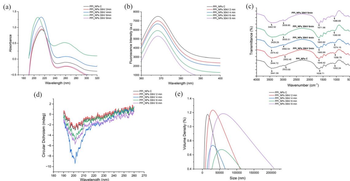
Fig. 1 Dielectric bather discharge cold plasma treatment of PPI-NPs as tested by (a) UV absorption spectra, (b) fluorescence absorption spectra and secondary structures reported by (c) FTIR analysis, (d) circular dichroism spectra, and (e) particle size.
