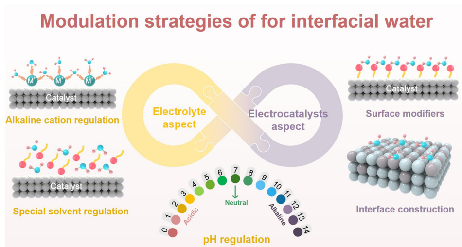
Fig. 9 Summary of modulation strategies of interfacial water for enhanced electrocatalytic performance.
