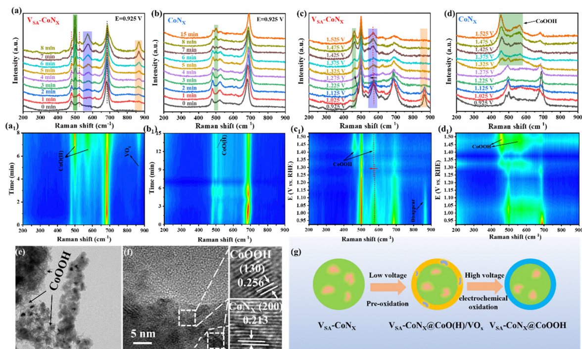
Fig. 4 Time-dependent in situ Raman spectra of (a) V SA -CoN x and (b) CoN x at a constant voltage. Potential-dependent in situ Raman spectra of (c) V SA -CoN x and (d) CoN x . (a 1 )–(d 1 ) The corresponding contour maps. (e) TEM and (f) HRTEM images of V SA -CoN x after the UOR stability test. (g) Schematic representation of active species in V SA -CoN x under different voltages.
