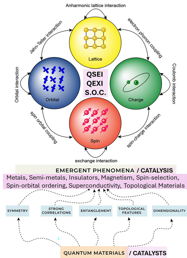
Fig. 1 Quantum materials show subtle quantum effects in controlling the macroscopic behaviour of materials, which also provide them with unique functionalities in catalysis. Adapted from https://www.jncasr.ac.in/faculty/abhishekkumar/research-area/ultrafast-physics-emerging-quantum-materials ; accessed 18/05/2025.
