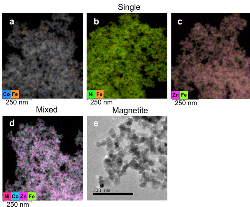
Fig. 3 Transmission electron micrographs of solid samples collected after sorption of Co(II), Ni(II) and Zn(II) on MNPs (5 g L -1 ) at pH 7 under anoxic conditions. Energy Dispersive X-ray spectroscopy (EDX) elemental mapping for single metal experiments show a) Co in blue b) Ni in green and c) Zn in pink covering the MNPs surface. In addition, Fig. 3d presents the mixed metal system where Co is blue, Ni is dark pink and Zn is light pink. Fig. 3e shows pure MNPs.
