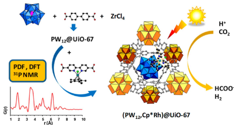
Fig. 6 Schematic diagram of the synthetic route and photocatalytic structure of the \text{Cp}^*\text{Rh@UiO-67} material. 106
