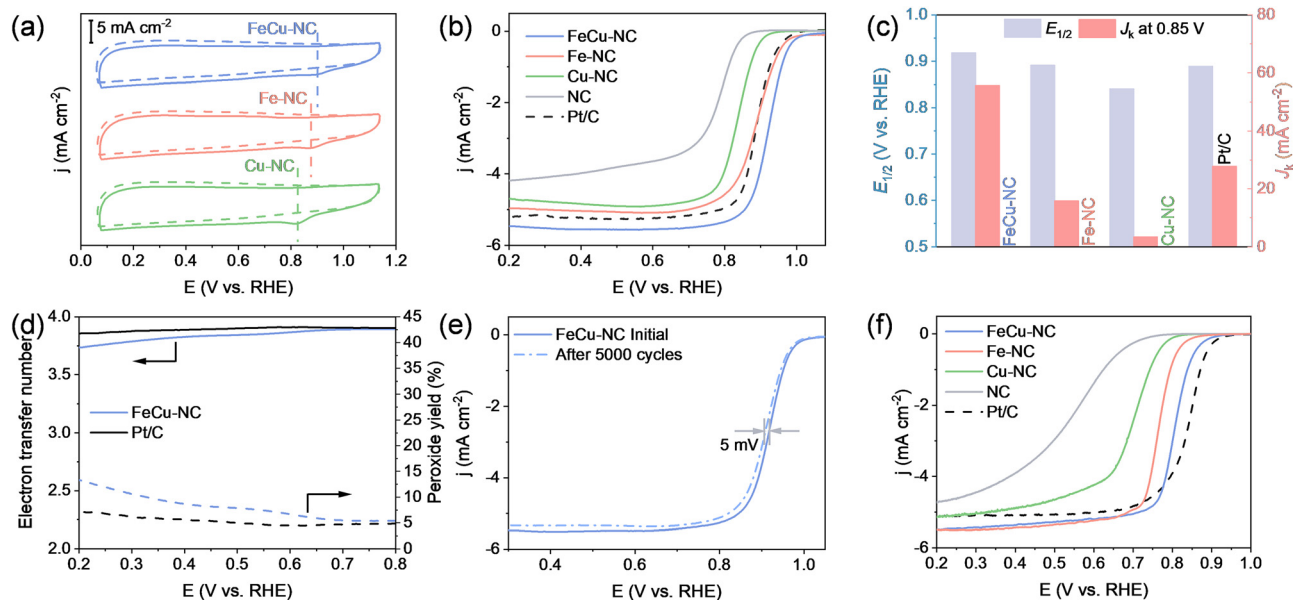
Fig. 3 (a) CV profiles of various catalysts in \text{O}_2 -saturated (solid line) or \text{N}_2 -saturated (dash line) 0.1 M KOH solution. (b) ORR polarization curves of different samples in \text{O}_2 -saturated 0.1 M KOH solution. (c) E_{1/2} and J_k at 0.85 V of different samples in 0.1 \text{O}_2 -saturated M KOH solution. (d) Peroxide yield and the corresponding electron transfer number for FeCu-NC and Pt/C determined by RRDE measurements in \text{O}_2 -saturated 0.1 M KOH solution. (e) ORR polarization curves of FeCu-NC before and after the durability test in 0.1 M KOH solution. (f) ORR polarization curves of different samples in \text{O}_2 -saturated 0.1 M \text{HClO}_4 solution.
