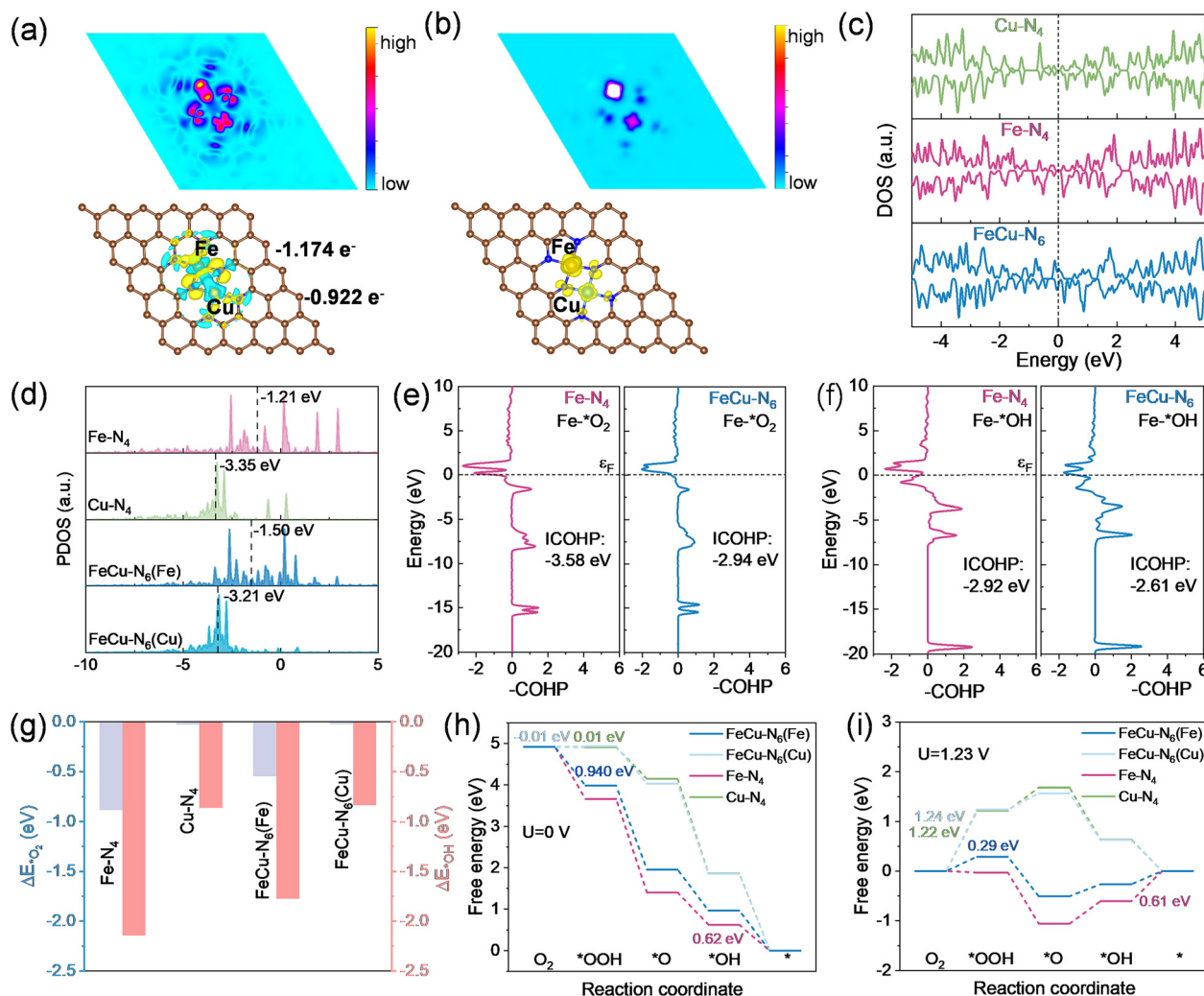
Fig. 4 (a) Bader charge analysis and visualization of charge density redistribution in FeCu-N6. (b) Spin density distribution and channel in FeCu-N6. (c) Density of states (DOS) of FeCu-N6, Fe-N4, and Cu-N4. (d) PDOS of d orbitals for metal sites in different models with corresponding d-band center positions indicated. (e) and (f) Analysis of the pCOHP between the Fe active sites in different models and oxygen atoms during (e) O2 adsorption and (f) *OH adsorption. (g) Adsorption energy of O2 and *OH on different metal active sites in various models. (h) and (i) Gibbs free energy diagrams for the ORR process in different models.
