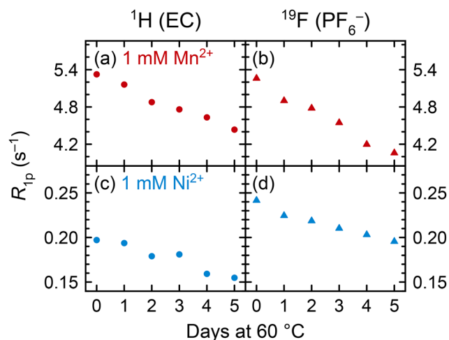
Fig. 4 (a) and (c) 1 H EC (circles) and (b) and (d) 19 F PF 6 - (triangles) longitudinal paramagnetic relaxation rates ( R_{1\text{p}} ) of Mn 2+ - or Ni 2+ - containing electrolyte solutions across five days of heating at 60 °C. Electrolyte solutions comprised 1 M LiPF 6 in 3:7 EC:EMC (v/v) with 1 mM Mn(TFSI) 2 (red) or Ni(TFSI) 2 (blue). Solutions were cooled to ambient temperature (~25 °C) before relaxation rates were measured.
