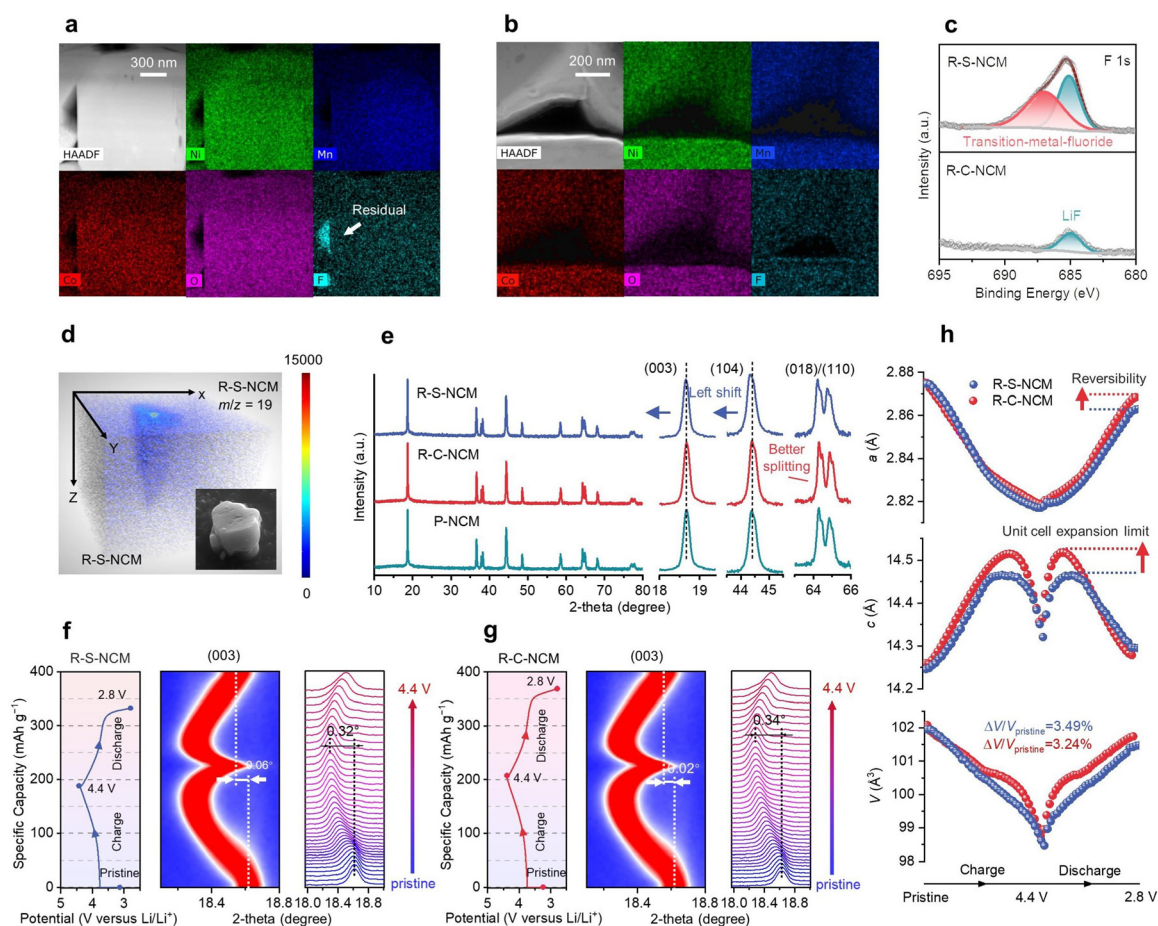
Fig. 3 Chemical and structural details of the regenerated cathode materials under the influence of impurities. (a) HAADF-STEM images and (b) corresponding EDS element mappings of R-S-NCM and R-C-NCM particles, focusing on the pores of the packing particles. (c) F 1s XPS high-resolution patterns of R-S-NCM and R-C-NCM powders. (d) Pseudo-three-dimensional distribution of F element and SEM image of the corresponding R-S-NCM particle. (e) Full patterns and characteristic peak comparison of the regenerated and pristine NCM cathodes with Cu K \alpha radiation at a scan rate of 8° min -1 . (f) 1st charge-discharge curves, corresponding XRD patterns of R-S-NCM, and (g) (003) peak position variation when the cell charge from pristine to 4.4 V and comparison with R-C-NCM. (h) Lattice parameters a , c , and the unit cell volume V of R-S-NCM and R-C-NCM in the 1st charge-discharge test according to the refinement.
