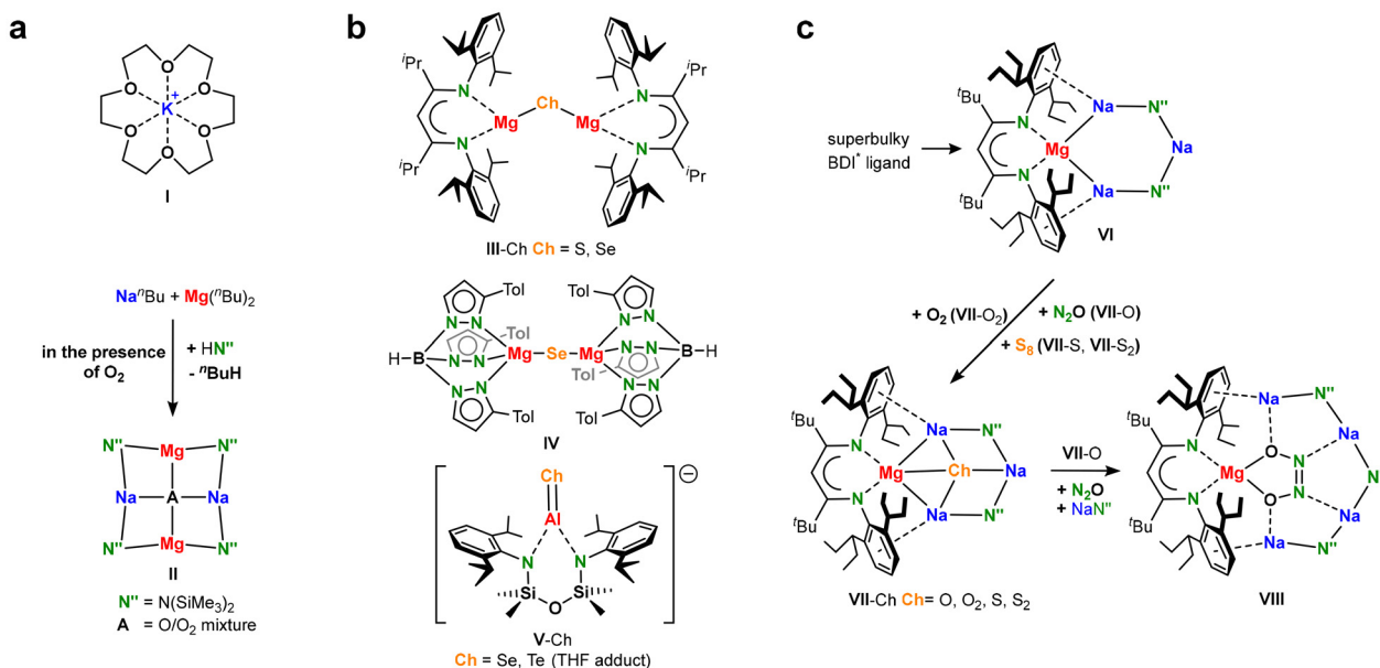
Scheme 1 (a) From Pedersen's crown ethers 1–3 to Mulvey's inverse crown complexes. 4–6 (b) Main group metal complexes with formal Ch – centres. 8–11 (c) The reduction of O 2 , N 2 O or S 8 with redox-active metal crown complex VI. 24
