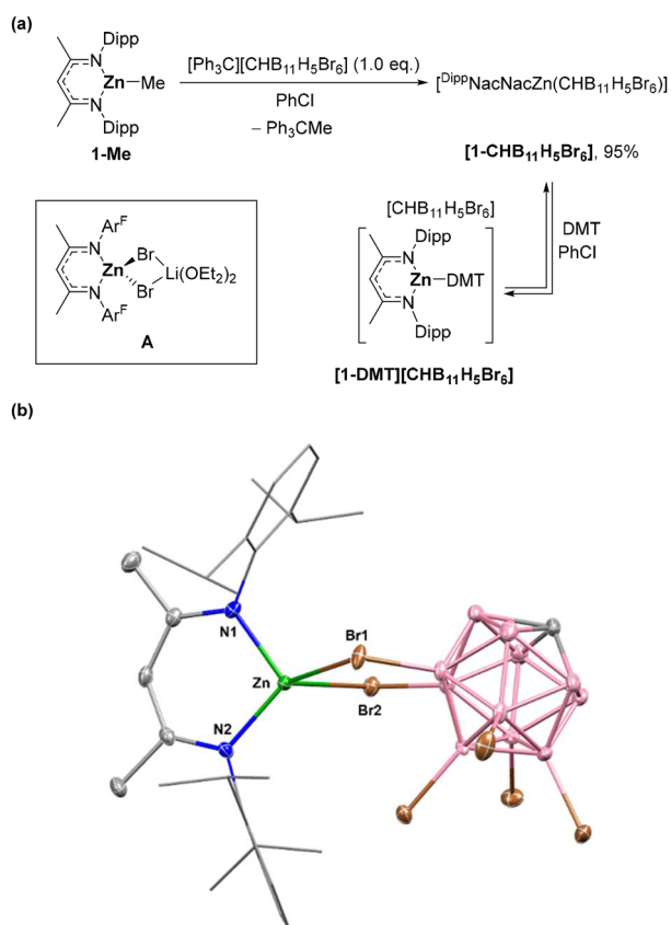
Fig. 3 (a) The formation of [1-CHB 11 H 5 Br 6 ] and its subsequent reaction with DMT; inset: structure of ArNacNacZn(μ-Br) 2 Li(OEt) 2 ( A ; Ar = 2,6-F 2 C 6 H 3 ). (b) Solid-state structure of [1-CHB 11 H 5 Br 6 ] ; ellipsoids are at 50% probability and H atoms are omitted for clarity. Selected bond distances (Å): Zn–N1 = 1.933(3), Zn–N2 = 1.925(5), Zn–Br1 = 2.519(8), Zn–Br2 = 2.571(1).
