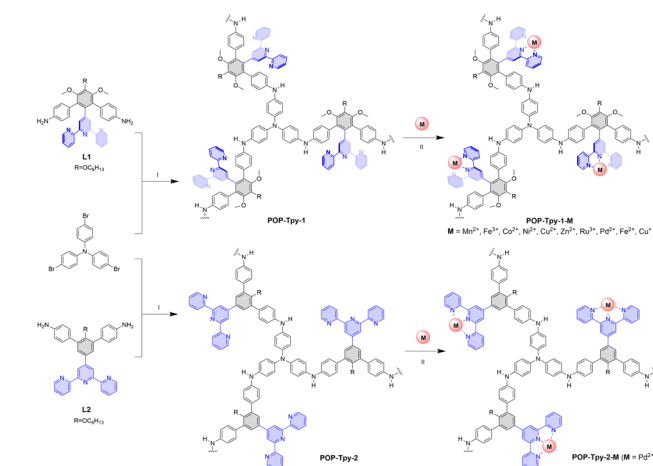
Scheme 1 Synthetic route of POP-Tpy-1/2 and POP-Tpy-1/2-M (reagents and conditions: (I) \text{Pd}(\text{dba})_2 , XPhos, \text{NaOtBu} , THF, 65^\circ\text{C} , 48 h; (II) MeOH or \text{CH}_2\text{Cl}_2/\text{CH}_3\text{CN} , metal salt).
