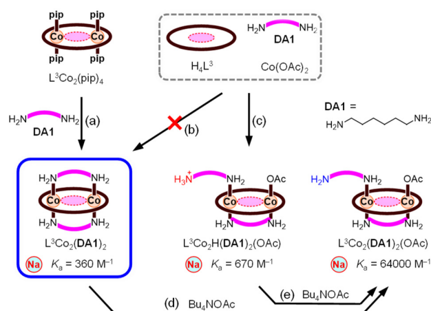
Fig. 11 Formation of doubly and singly bridged metallohosts with the 1,6-hexanediamine ligand ( DA1 ) based on the L^3Co_2 macrocycle.
