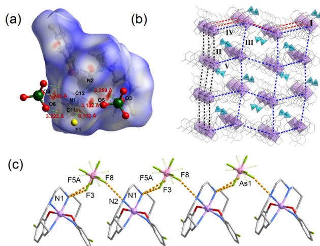
Fig. 4 (a) Hirshfeld surface analysis of complex 1 at 60 K, showing the d_{norm} surfaces of the mono-cationic unit. (b) Crystal packing of complex 1 at 300 K, viewed along the a axis. (c) View of the 1D hydrogen-bond chain of complex 2.
