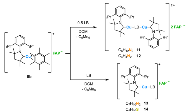
Scheme 2 Synthesis of [(\text{cAAC}^{\text{Me}})\text{Cu}]_2(\text{C}_6\text{H}_{12}\text{N}_2)]^{2+} \cdot 2\text{FAP}^- ( 11 ), [(\text{cAAC}^{\text{Me}})\text{Cu}]_2(\text{C}_4\text{H}_4\text{N}_2)]^{2+} \cdot 2\text{FAP}^- ( 12 ), [(\text{cAAC}^{\text{Me}})\text{Cu}(\text{C}_7\text{H}_{10}\text{N}_2)]^+ \cdot \text{FAP}^- ( 13 ), and [(\text{cAAC}^{\text{Me}})\text{Cu}(\text{C}_4\text{H}_{10}\text{S})]^+ \cdot \text{FAP}^- ( 14 ) via hexamethylbenzene substitution of [(\text{cAAC}^{\text{Me}})\text{Cu}(\text{C}_6\text{Me}_6)]^+ \cdot \text{FAP}^- ( IIb ).
