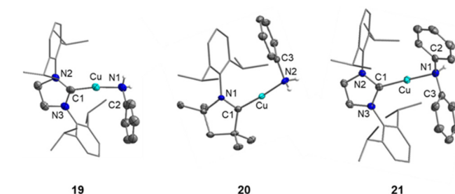
Fig. 5 Molecular structures of the complex cations of [(SIDipp)Cu(NH 2 Ph)] + FAP − ( 19 , left), [(cAAC Me )Cu(NH 2 Ph)] + FAP − ( 20 , middle) and [(IDipp)Cu(NHPh 2 )] + FAP − ( 21 , right) in the solid state (ellipsoids set at the 50% probability level; Dipp substituents are shown as wire-and-stick models). Hydrogen atoms except for those of the N atom of the aniline and diphenylamine ligands and a solvent molecule in the crystal structure of 19 are omitted for clarity. Only one of two independent cations in the asymmetric unit of 19 is shown. Selected bond lengths and angles are collected in Table 2 and Fig. S11–S13 in the ESI.†
