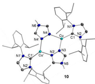
Fig. 2 Molecular structure of the complex cation of [(\text{IDipp})\text{Cu}]_2(\text{C}_2\text{N}_3\text{H}_3)_2]^{2+} \cdot 2\text{FAP}^- ( 10 ) in the solid state (ellipsoids set at the 50% probability level; Dipp substituents are shown as wire-and-stick models). Hydrogen atoms except for the ones bound to N5 and N6 and a co-crystallized solvent molecule are omitted for clarity. Selected bond length and angles are collected in Table 2 and Fig. S6 in the ESI.†
