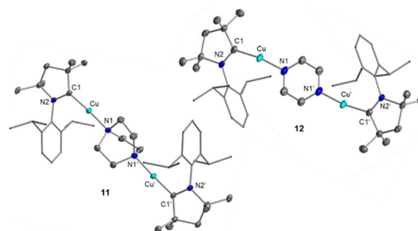
Fig. 3 Molecular structures of the complex cations of [(\text{cAAC}^{\text{Me}})\text{Cu}]_2(\text{C}_6\text{H}_{12}\text{N}_2)]^{2+} \cdot 2\text{FAP}^- ( 11 ; left) and [(\text{cAAC}^{\text{Me}})\text{Cu}]_2(\text{C}_4\text{H}_4\text{N}_2)]^{2+} \cdot 2\text{FAP}^- ( 12 ; right) in the solid state (ellipsoids set at the 50% probability level; Dipp ligands are shown as wire-and-stick models). Hydrogen atoms are omitted for clarity. Selected bond length and angles are collected in Table 2 and Fig. S7, S8 in the ESI.†
