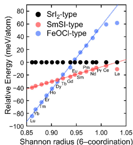
Fig. 3 Relative energy of the \text{SmSI} - and \text{FeOCl} -type structures with respect to the \text{SrI}_2 -type structure as a function of the Shannon radius of the \text{Ln}^{3+} cation. Note that both the \text{SrI}_2 - and \text{SmSI} -type structures exhibit seven-fold coordination around the Ln cation; however, we use the ionic radii of six-fold coordination to facilitate comparison.
