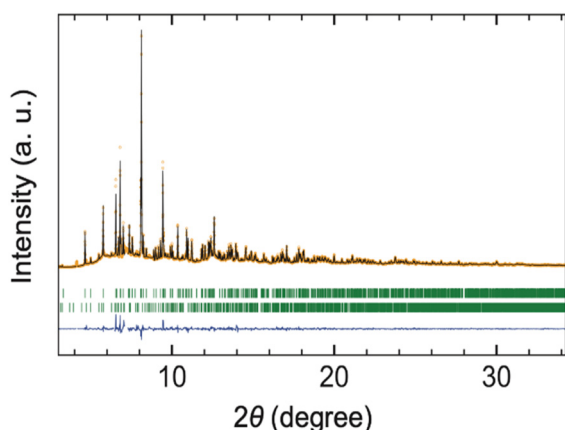
Fig. 2 Rietveld refinement of SXRD data collected for LaSI ( \lambda = 0.420201 \text{ \AA} ), adopting the \text{SrI}_2 -type structure with space group Pcab . Orange circles, black lines, and blue lines represent the observed, calculated, and residual intensity, respectively. The green ticks indicate the Bragg reflection positions for LaSI (upper) and \text{La}_{10}\text{OS}_{14} (lower). The weight fraction of \text{La}_{10}\text{OS}_{14} is 13.6(2)%.
