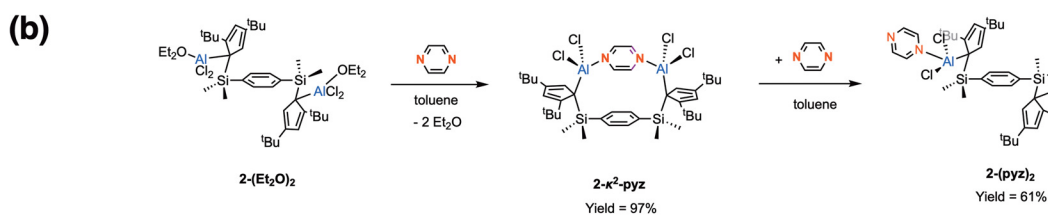
Scheme 2 Reactivity of (a) 1-(Et 2 O) 2 and (b) 2-(Et 2 O) 2 .
