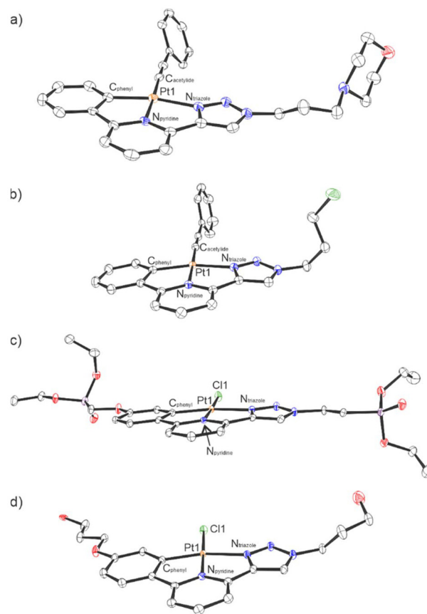
Fig. 2 Molecular structures of (a) [\text{Pt}(\text{A})^M\text{L}] , (b) [\text{Pt}(\text{A})^{\text{Cl}}\text{L}] (a co-crystallized \text{CH}_2\text{Cl}_2 molecule is omitted for clarity), (c) [\text{PtCl}^{\text{P}}\text{L}^{\text{P}}] , and (d) [\text{PtCl}^{\text{OH}}\text{L}^{\text{OH}}] (a co-crystallized DMF molecule (half a molecule in the asymmetric unit) is omitted for clarity) in the crystal. Displacement ellipsoids are drawn at the 50% probability level. H atoms are omitted for clarity.
