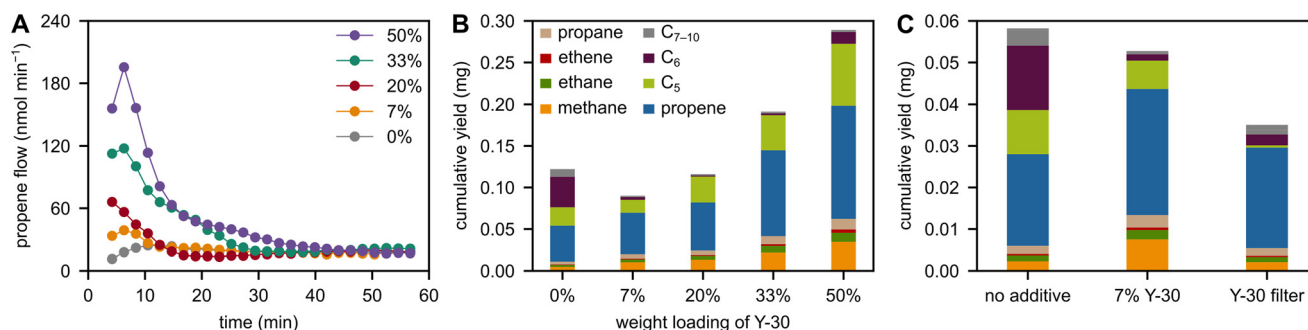
Fig. 1 (A) Propene flow during milling of PP with 6 Fe spheres at 30 Hz with 0–50 wt% of Y-30. (B) C_{1-10} hydrocarbon yield obtained after 1 h of milling PP with 6 Fe spheres at 30 Hz with 0–50 wt% of Y-30. (C) C_{1-10} hydrocarbon yield obtained after 0.5 h of milling PP with 6 Fe spheres at 30 Hz under three conditions: (i) without Y-30, (ii) with 7 wt% Y-30, and (iii) without any Y-30 in the reactor, but a Y-30 filter downstream of it.
