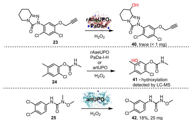
Scheme 5 UPO transformations of halogenated aromatics.
