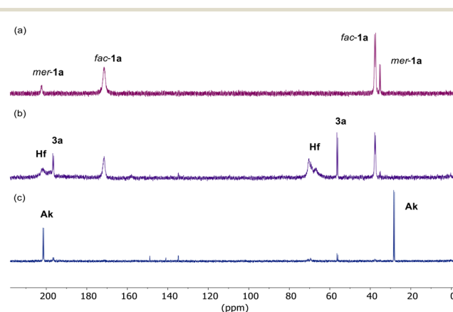
Fig. 6 31 P{ 1 H} NMR (202 MHz, toluene- d 8 ): spectra of 1a (a), activated 1a by reaction with H 2 and KOtBu after 15 min sonication (b), reaction of the latter with benzophenone (5 equiv., c).
