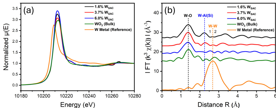
Fig. 5 (a) Normalized W L_{3\text{-edge}} X-ray absorption near-edge structure (XANES) spectra and (b) k^3 -weighted Fourier transform (FT) of the EXAFS spectra of 1.6–6.0% W_{SAC}/SDA , bulk WO_3 , and reference W metal samples.
